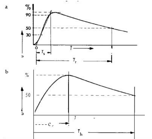
Fig. 4 Standardized test voltages a Lightning impulse voltage 1.2/50 Front time: T_s = 1.2 \pm 0.36 \mu s Time of half value: T_r = 50 \pm 10 \mu s b Switching impulse voltage 250/2500 Front time: T_{cr} = 250 \pm 50 \mu s Time of half value: T_h = 2500 \pm 1500 \mu s
